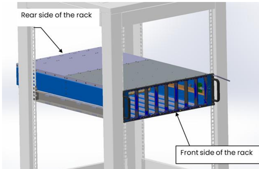
Figure 4: Mounted OPX1000 chassis
