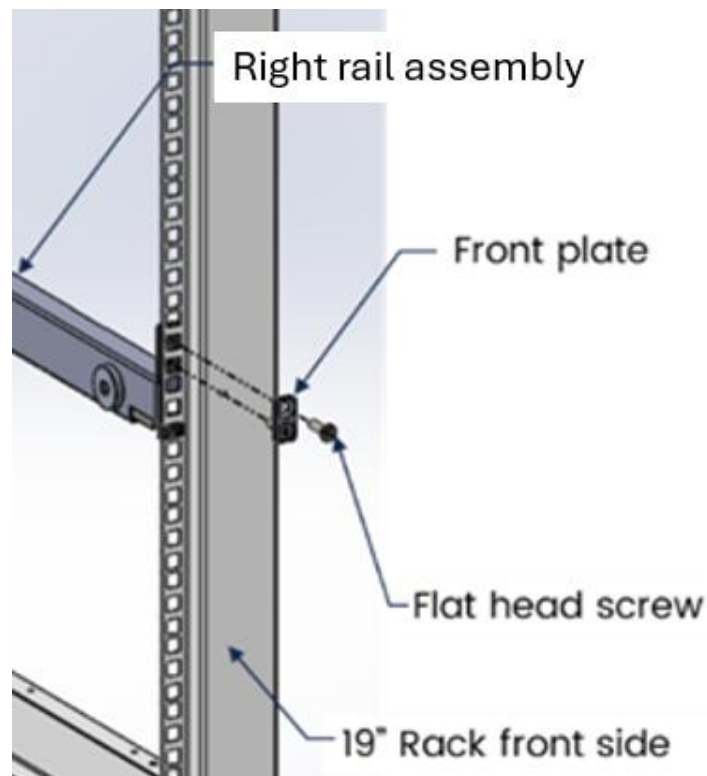
Figure 2 – Rail assembly and front plate installation
