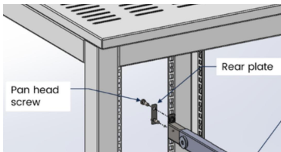
Figure 3 – Rail assembly and back plate installation
