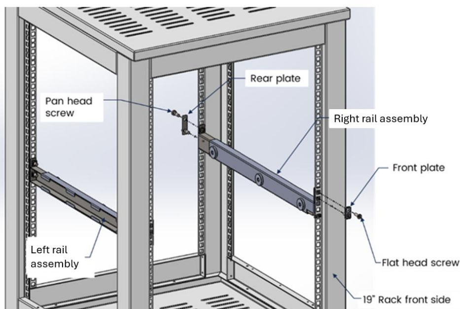
Figure 1 – Rack Mounting Kit Main Components
